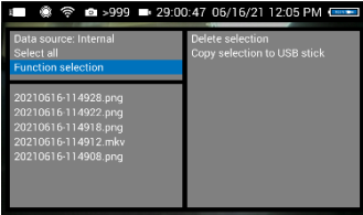
Fig. 24: Delete selected files
