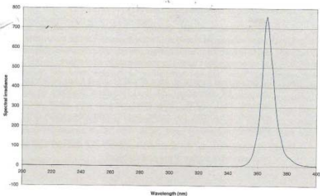
Figure 1. Mean spectral irradiance of Torch A at 100 cm (mW m -2 nm -1 )
